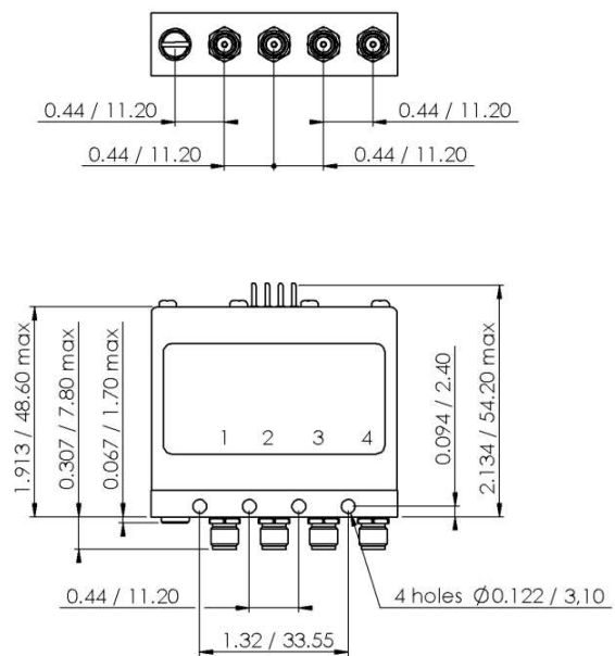
Model 26.5 GHz with solder pins
