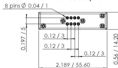
TOP view - solder pins
