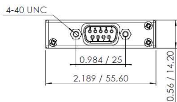
TOP view - D-Sub connector
