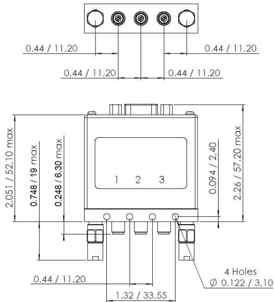
TOP view - D-Sub connector
