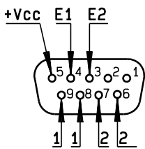
D-Sub connector
