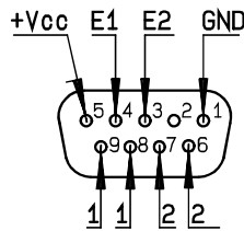
D-Sub connector
