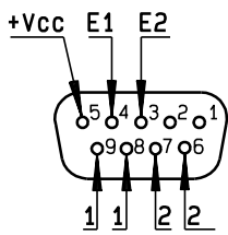
D-Sub connector
