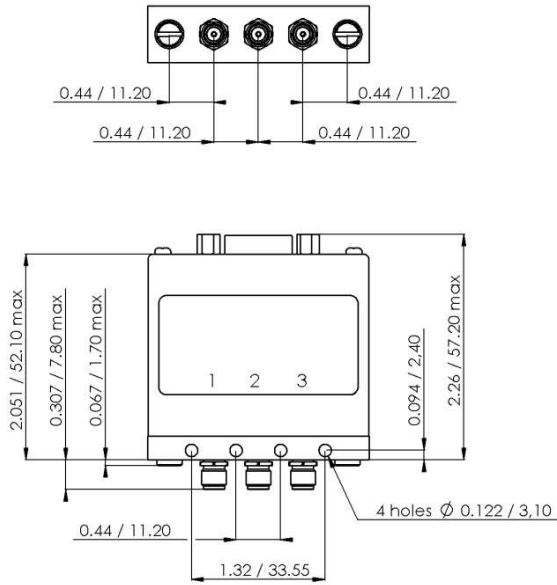
Model 40 GHz with D-Sub connector
