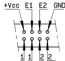
Solder pins
