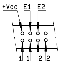
Solder pins
