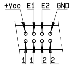
Solder pins
