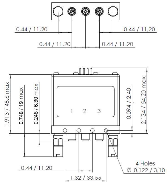
TOP view - solder pins
