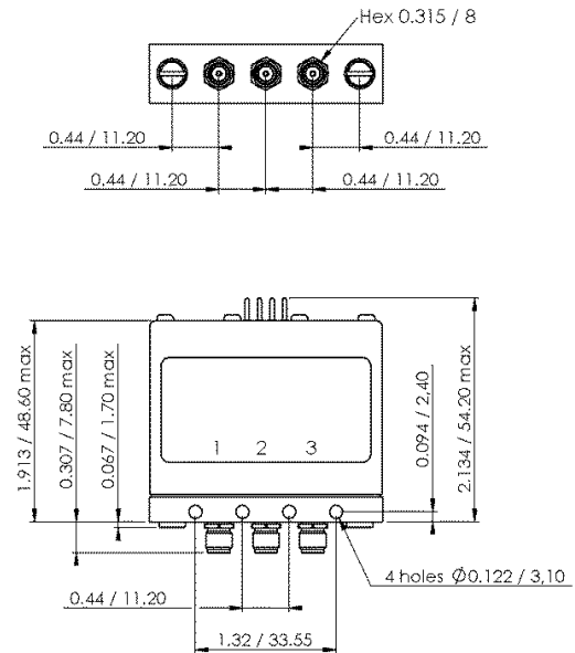
Model 40 GHz with solder pins
