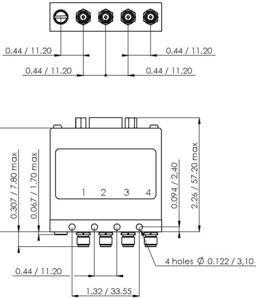
Model 26.5 GHz with D-Sub connector
