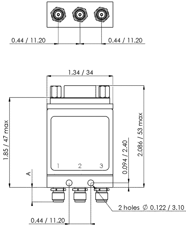
With D-Sub connector
