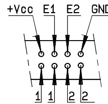
Solder pins
