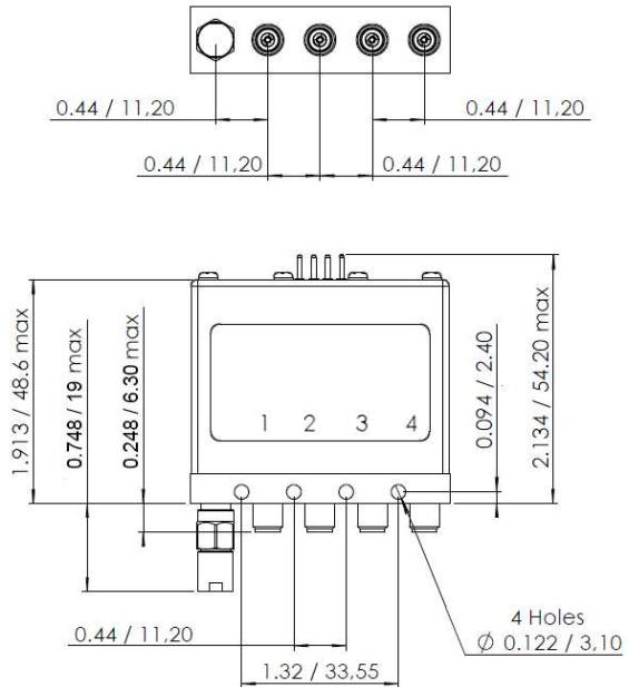
Model 40 GHz with solder pins
