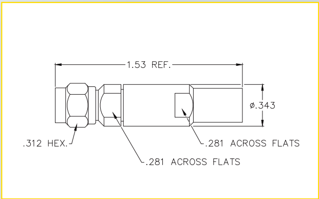
SMA MALE (SPS-1503)
