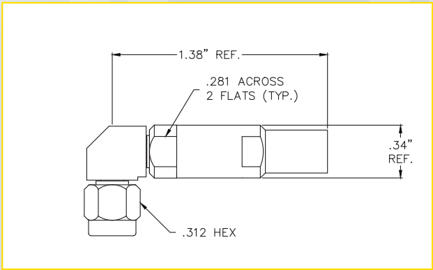
SMA MALE RIGHT ANGLE (SPRC-1503)
