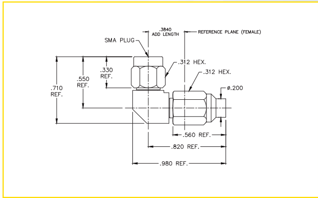
SMA MALE RIGHT ANGLE (SPRC-1501)
