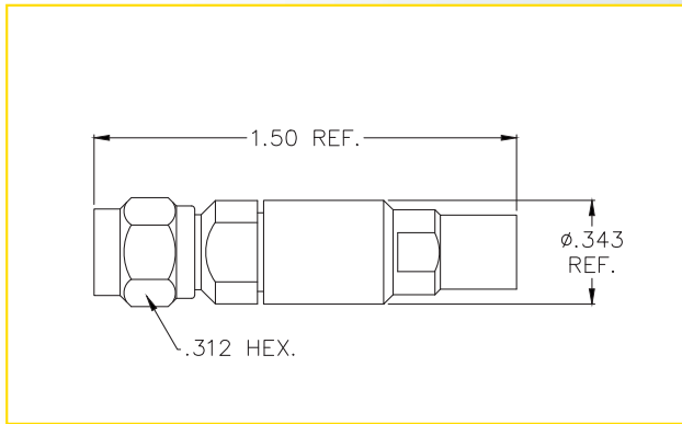
SMA MALE (SPS-1501)
