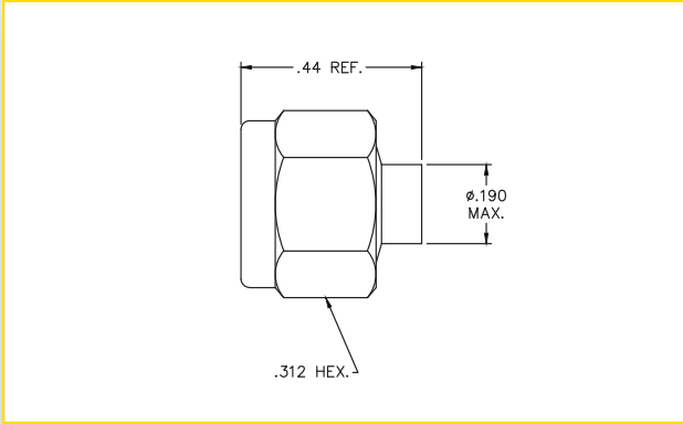
SMA MALE (SPSD-TPRF085)
