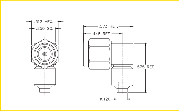
SMA MALE RIGHT ANGLE (SPRCD-TPRF085)
