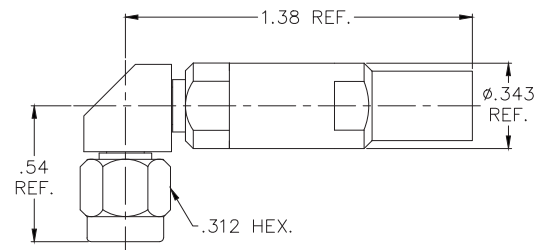
2.92MM RIGHT ANGLE MALE (KPR-1503)
