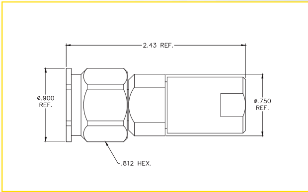
SC MALE (SCPS-4806)
