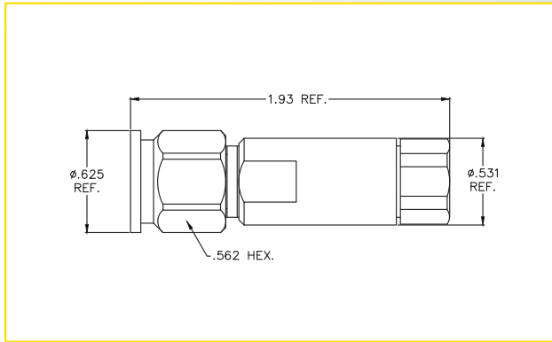
TNC MALE (TPS-2803)
