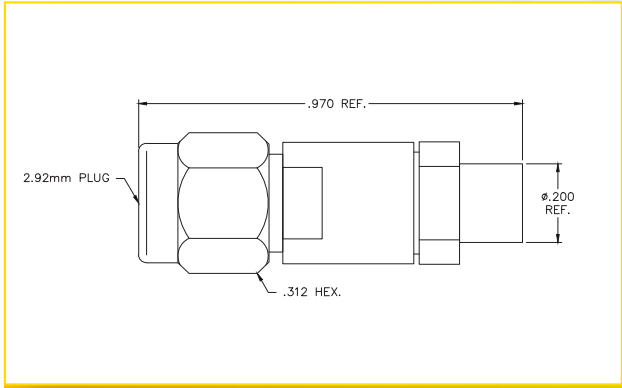
2.92MM MALE, LC JACKET (KPS-1501LC)
