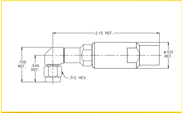
SMA MALE RIGHT ANGLE (SPRC-2801)
