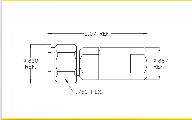
N-TYPE MALE (NPS-4806)
