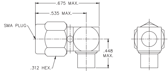
SMA MALE RIGHT ANGLE DIRECT SOLDER (SPRCD-TPRF141)
