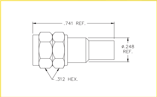
1.85MM MALE SHELL STYLE FOR EXTERNAL ARMOR (VJS-1251A)
