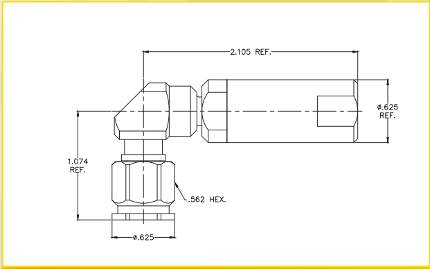
TNC MALE RIGHT ANGLE (TPR-2801)
