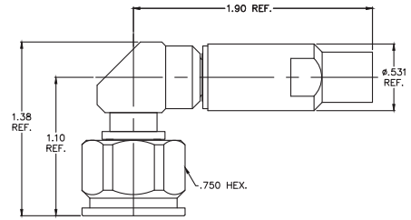
N-TYPE MALE RIGHT ANGLE (NPR-2801)
