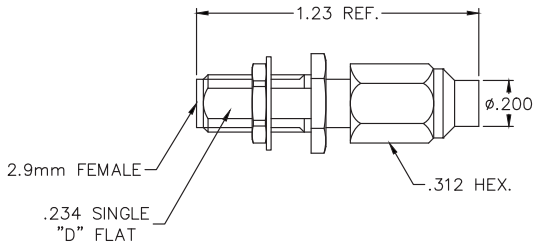
2.92MM FEMALE BULKHEAD (KJB-1501)
