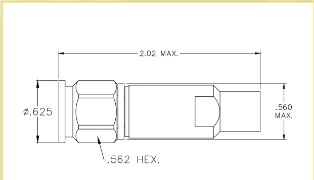
TNC MALE (TPS-2801)
