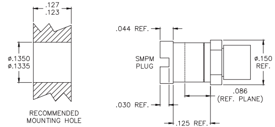
GPO MALE BULKHEAD (GGPB-TPRF085)
