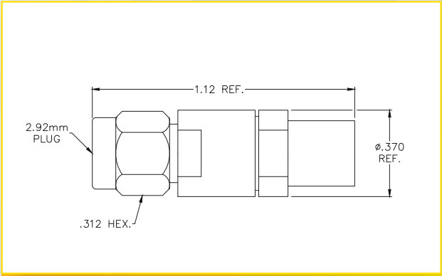
2.92MM MALE (KPS-1503)
