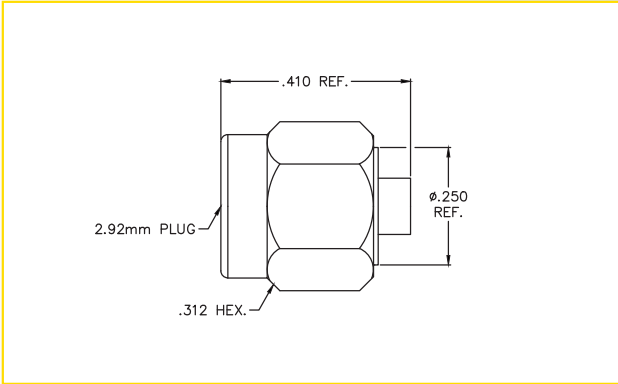
2.92MM MALE (KPSD-TPRF085)
