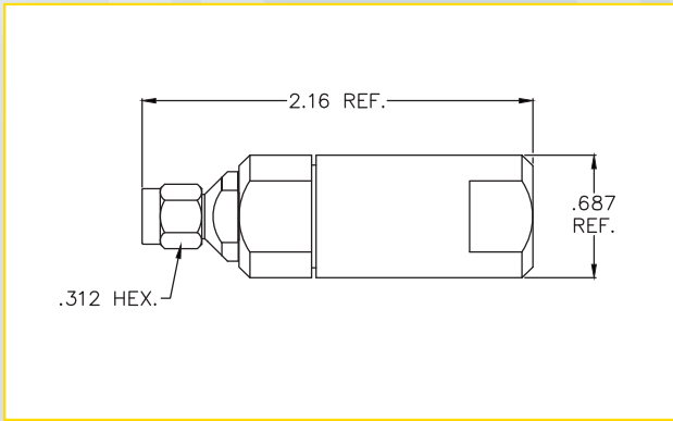
SMA MALE (SPS-4806)
