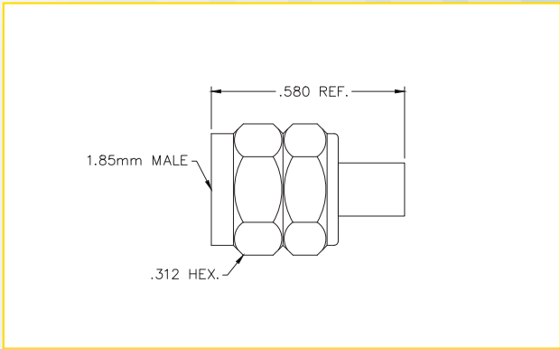
1.85MM MALE SHELL STYLE (VPSH-1251)
