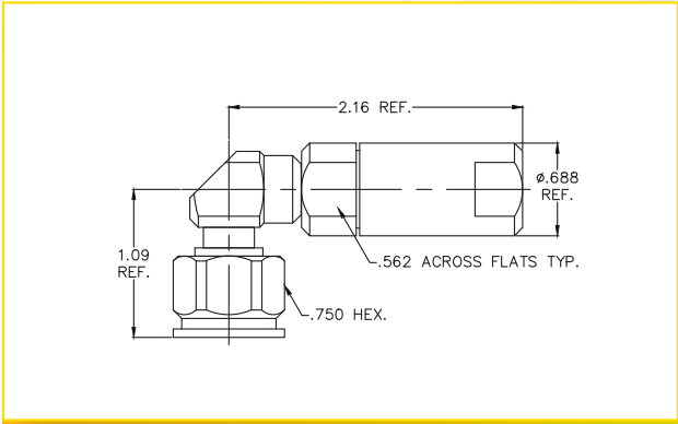
N-TYPE MALE RIGHT ANGLE (NPR-4806)
