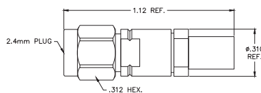
2.4MM MALE (2PS-1571)
