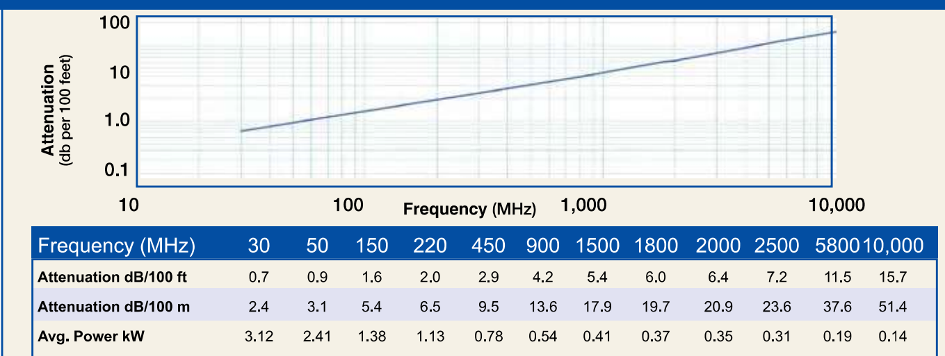
Attenuation vs. Frequency (typical)
